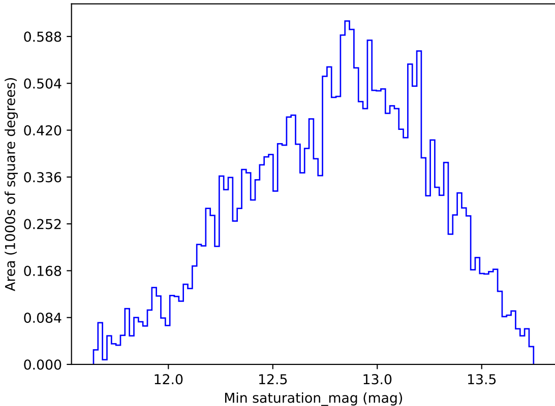
too_elab_r8_d2_griz_v3.4_10yrs All sky g band: Min saturation_mag
