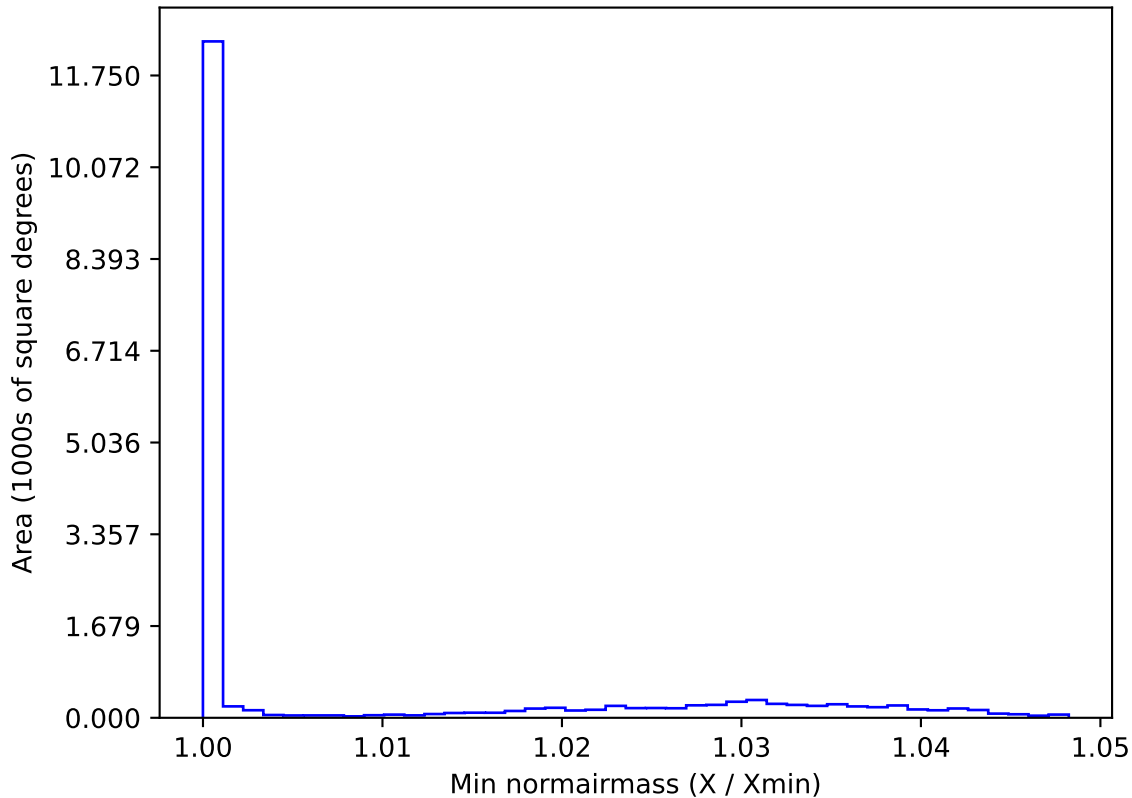
too_elab_r8_d2_griz_v3.4_10yrs WFD g band: Min normairmass
