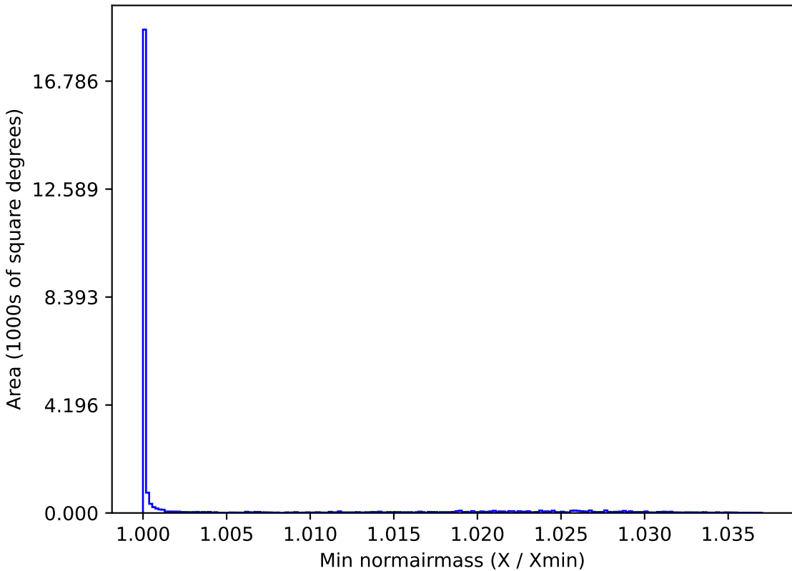
too_elab_r8_d2_griz_v3.4_10yrs All sky r band: Min normairmass
