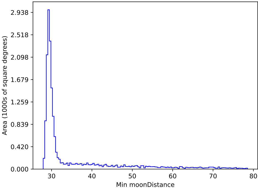
too_elab_r8_d2_griz_v3.4_10yrs WFD y band: Min moonDistance
