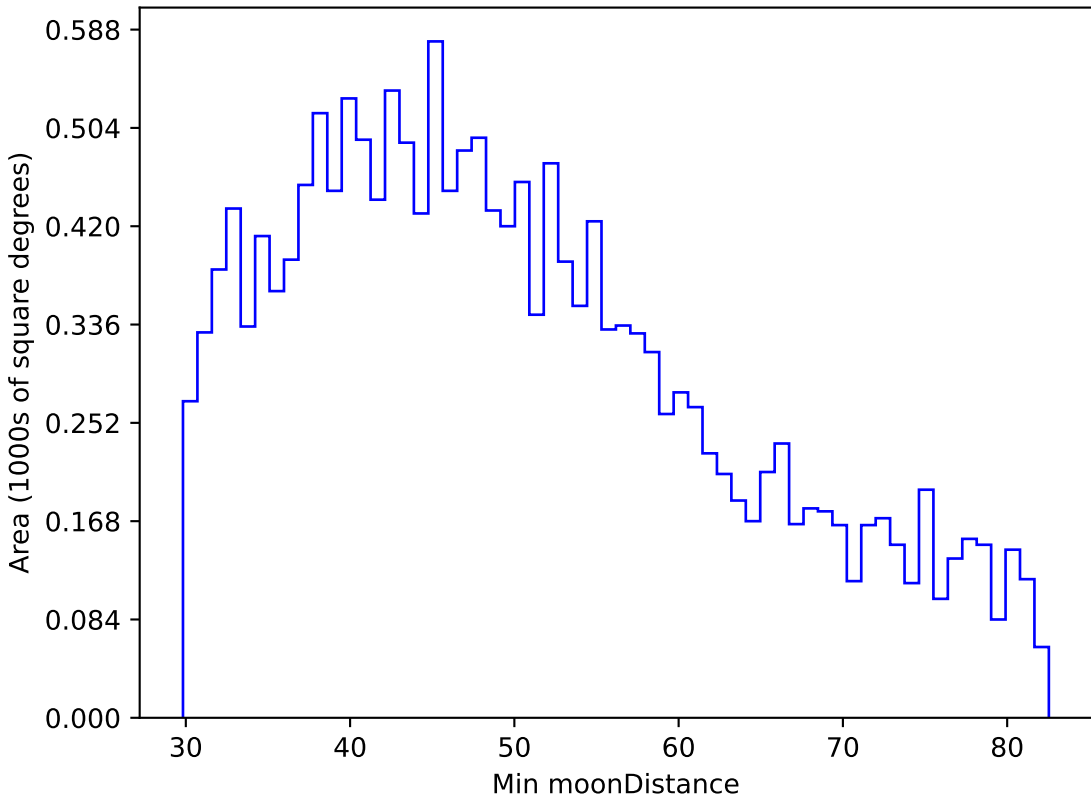
too_elab_r8_d2_griz_v3.4_10yrs WFD u band: Min moonDistance
