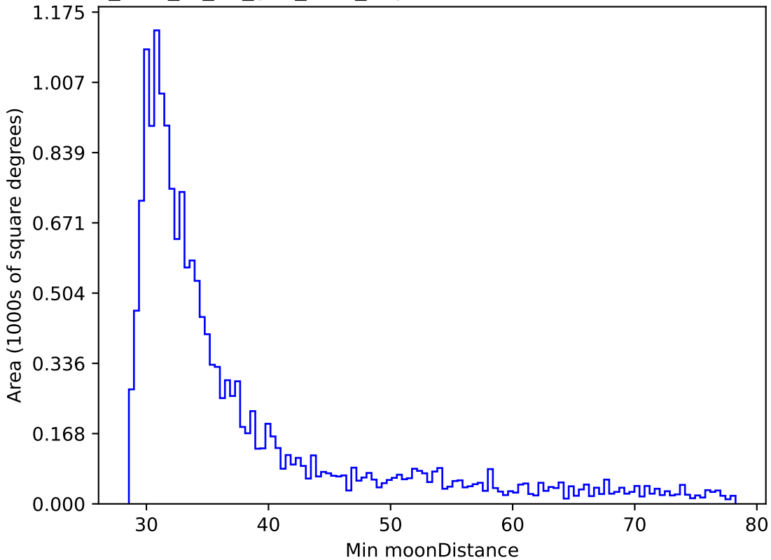
too_elab_r8_d2_griz_v3.4_10yrs WFD r band: Min moonDistance
