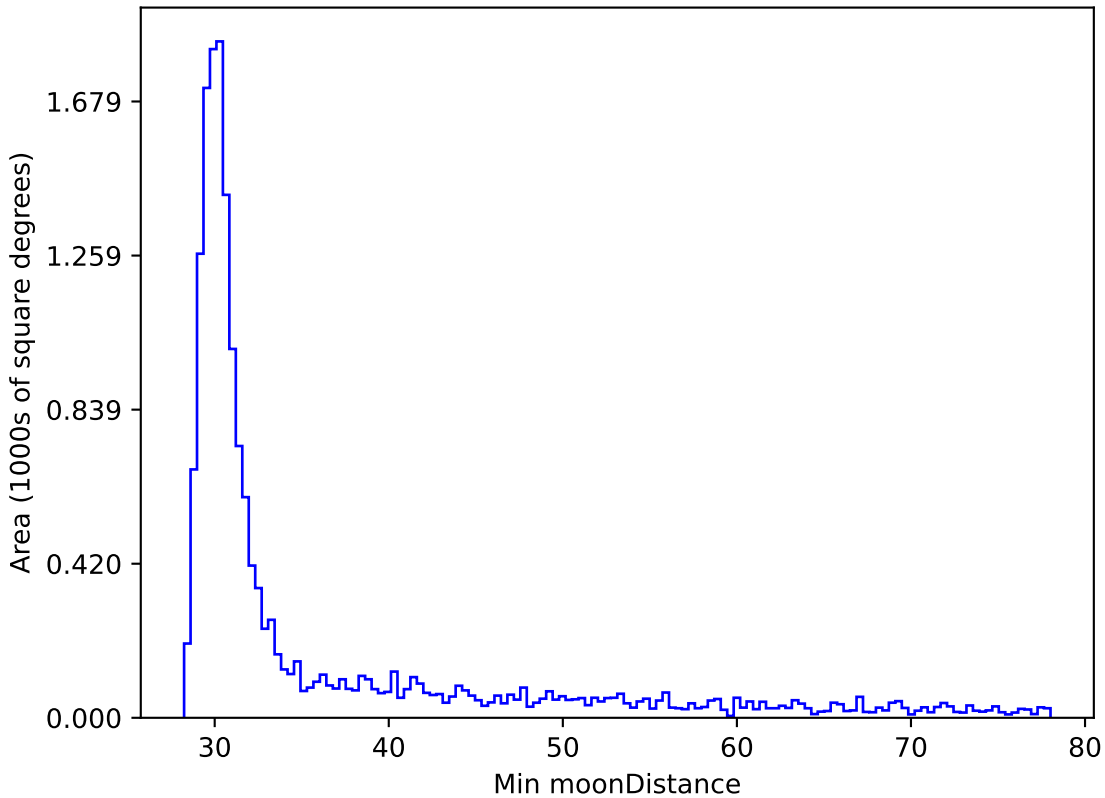
too_elab_r8_d2_griz_v3.4_10yrs WFD i band: Min moonDistance
