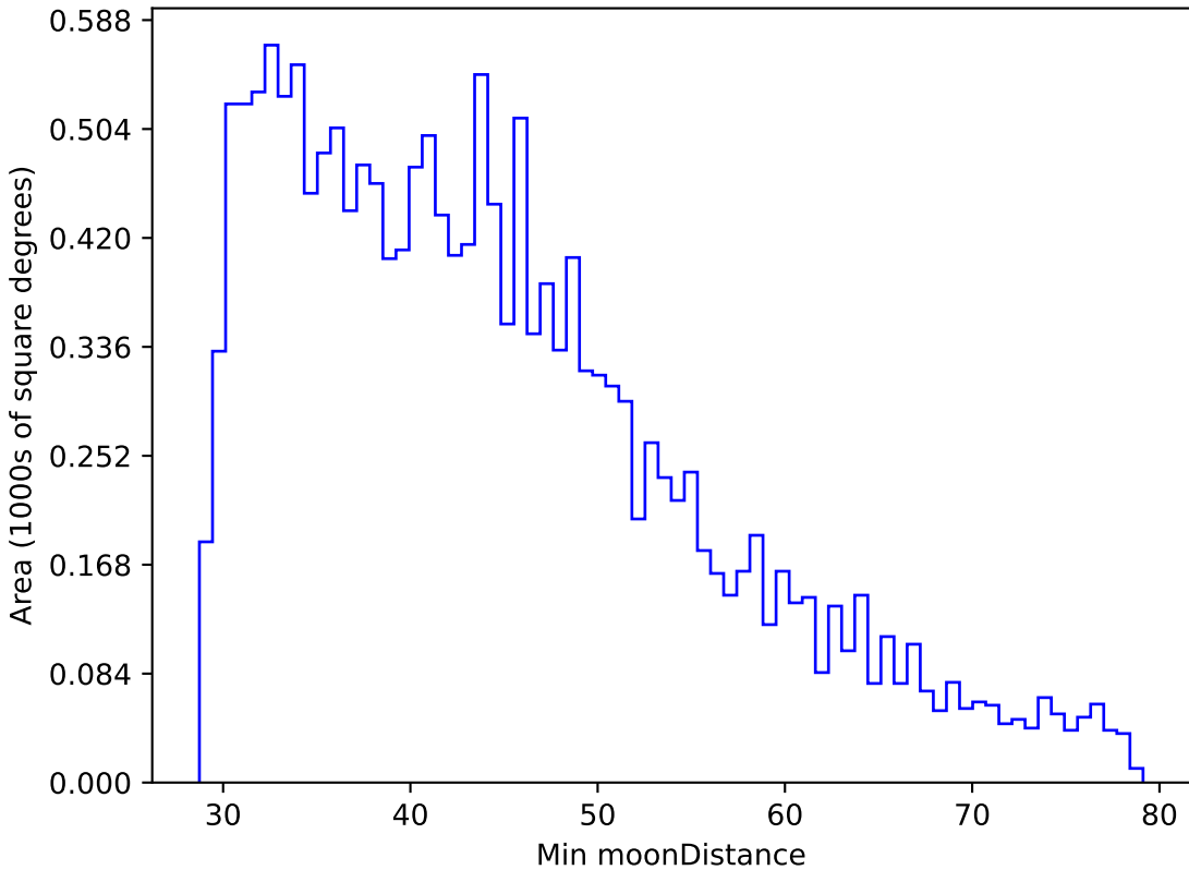
too_elab_r8_d2_griz_v3.4_10yrs WFD g band: Min moonDistance
