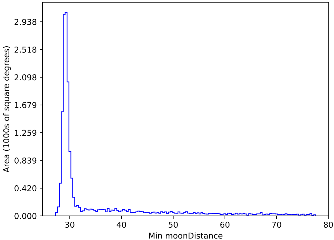
too_elab_r8_d2_griz_v3.4_10yrs WFD all bands: Min moonDistance
