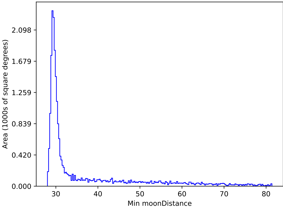
too_elab_r8_d2_griz_v3.4_10yrs All sky y band: Min moonDistance
