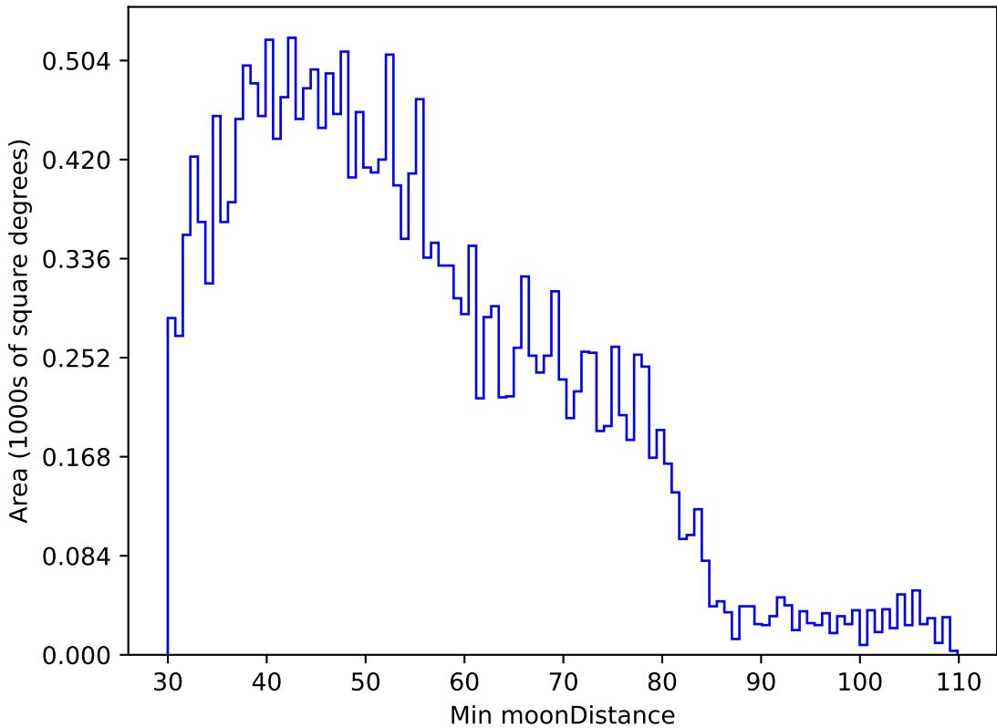
too_elab_r8_d2_griz_v3.4_10yrs All sky u band: Min moonDistance
