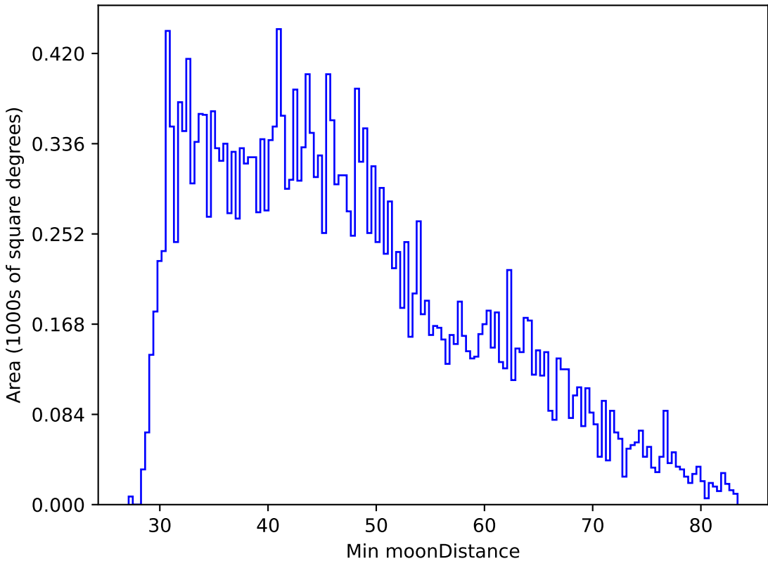
too_elab_r8_d2_griz_v3.4_10yrs All sky g band: Min moonDistance
