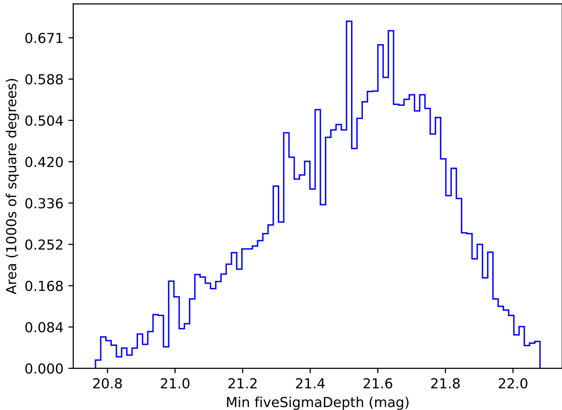
too_elab_r8_d2_griz_v3.4_10yrs Yr 1 y band: Min fiveSigmaDepth
