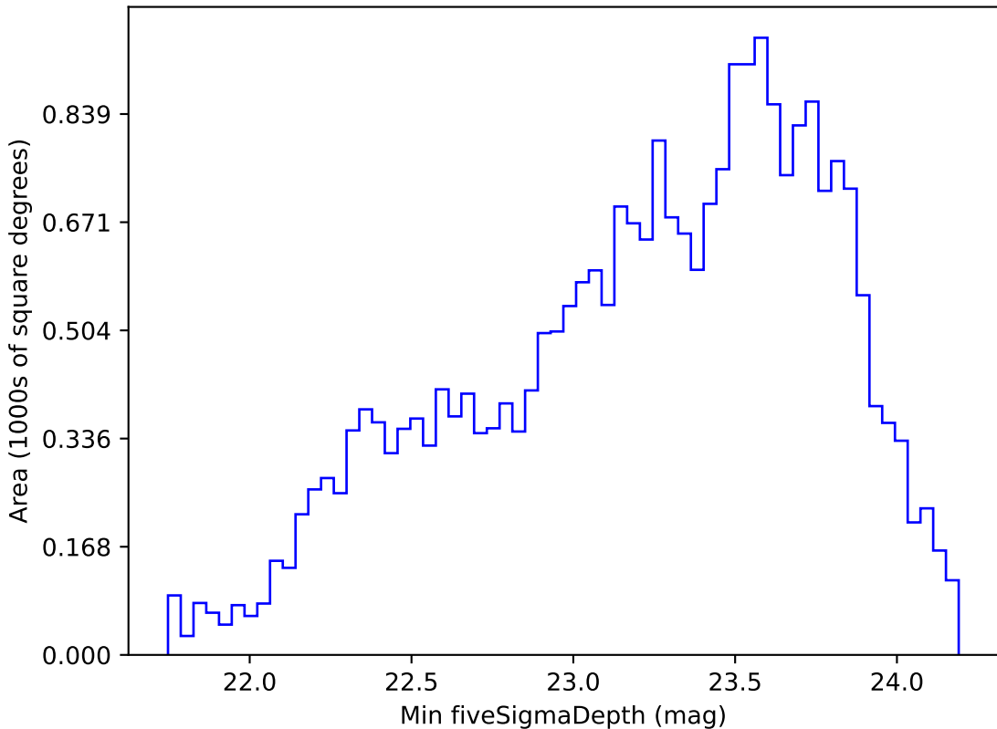
too_elab_r8_d2_griz_v3.4_10yrs Yr 1 r band: Min fiveSigmaDepth
