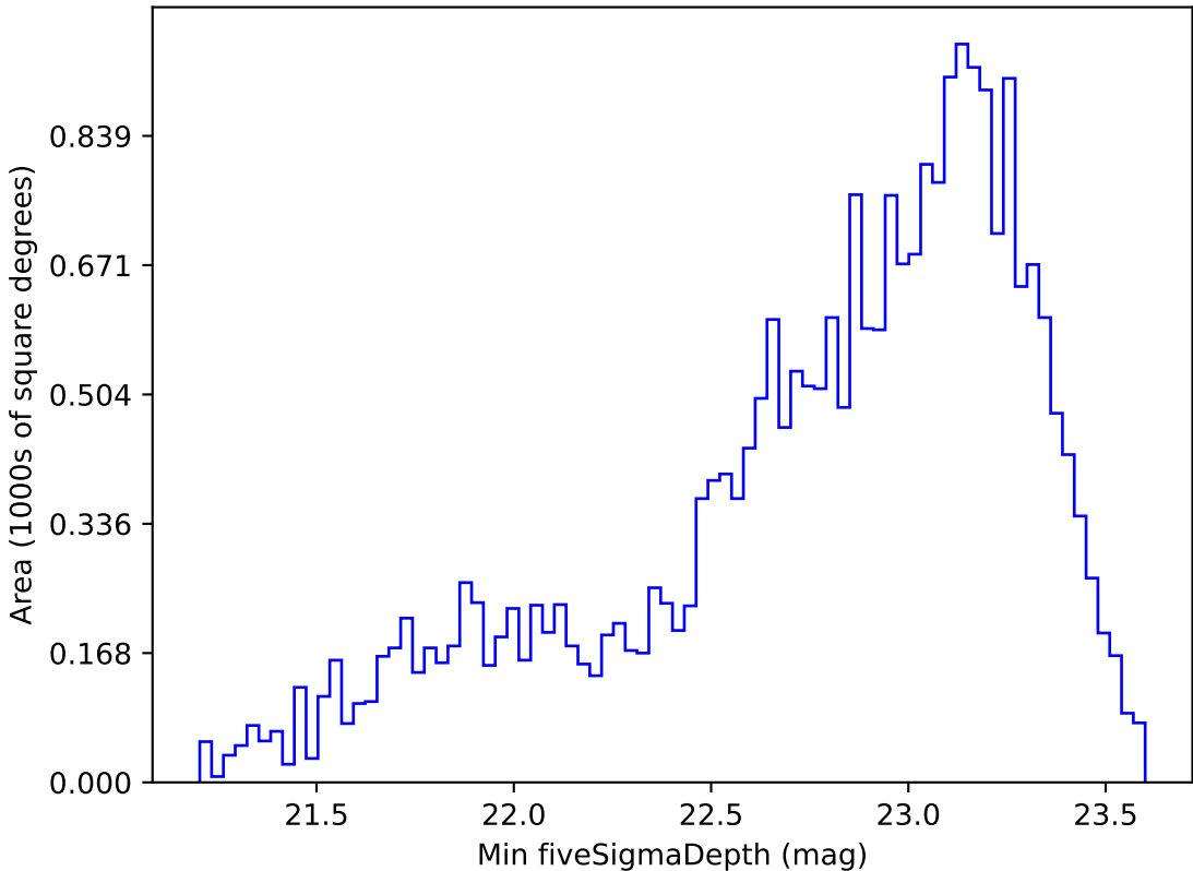
too_elab_r8_d2_griz_v3.4_10yrs Yr 1 i band: Min fiveSigmaDepth
