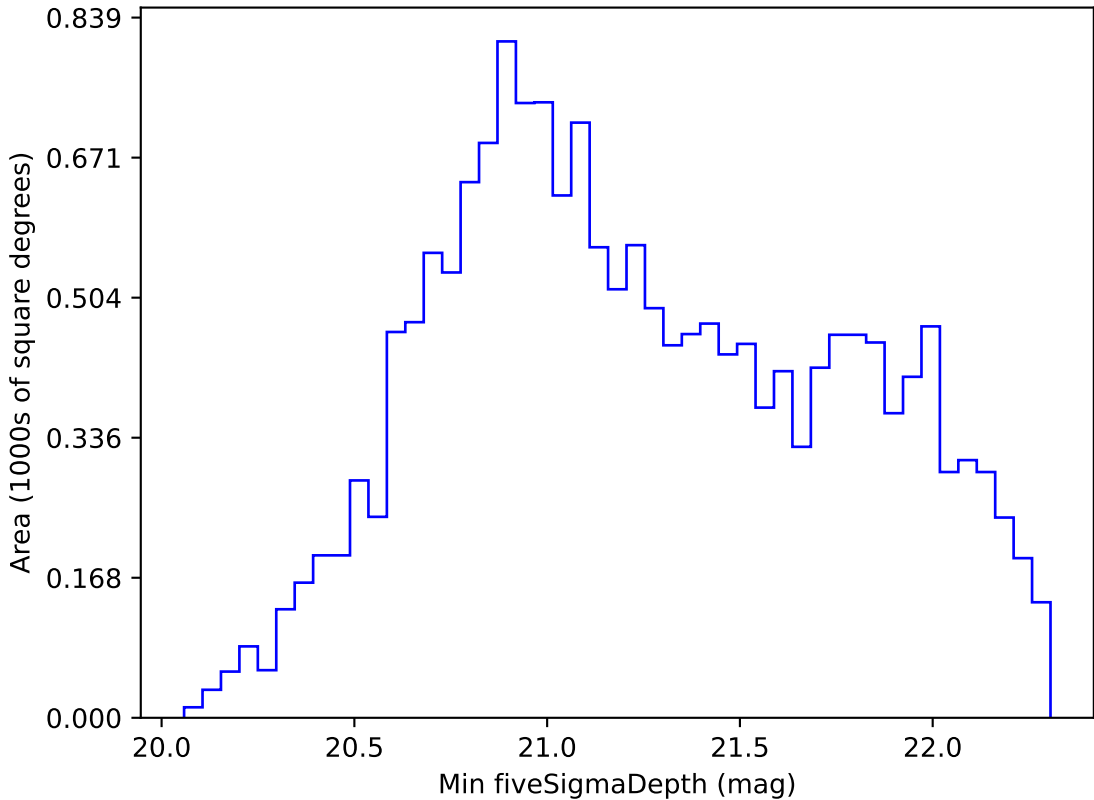
too_elab_r8_d2_griz_v3.4_10yrs WFD z band: Min fiveSigmaDepth
