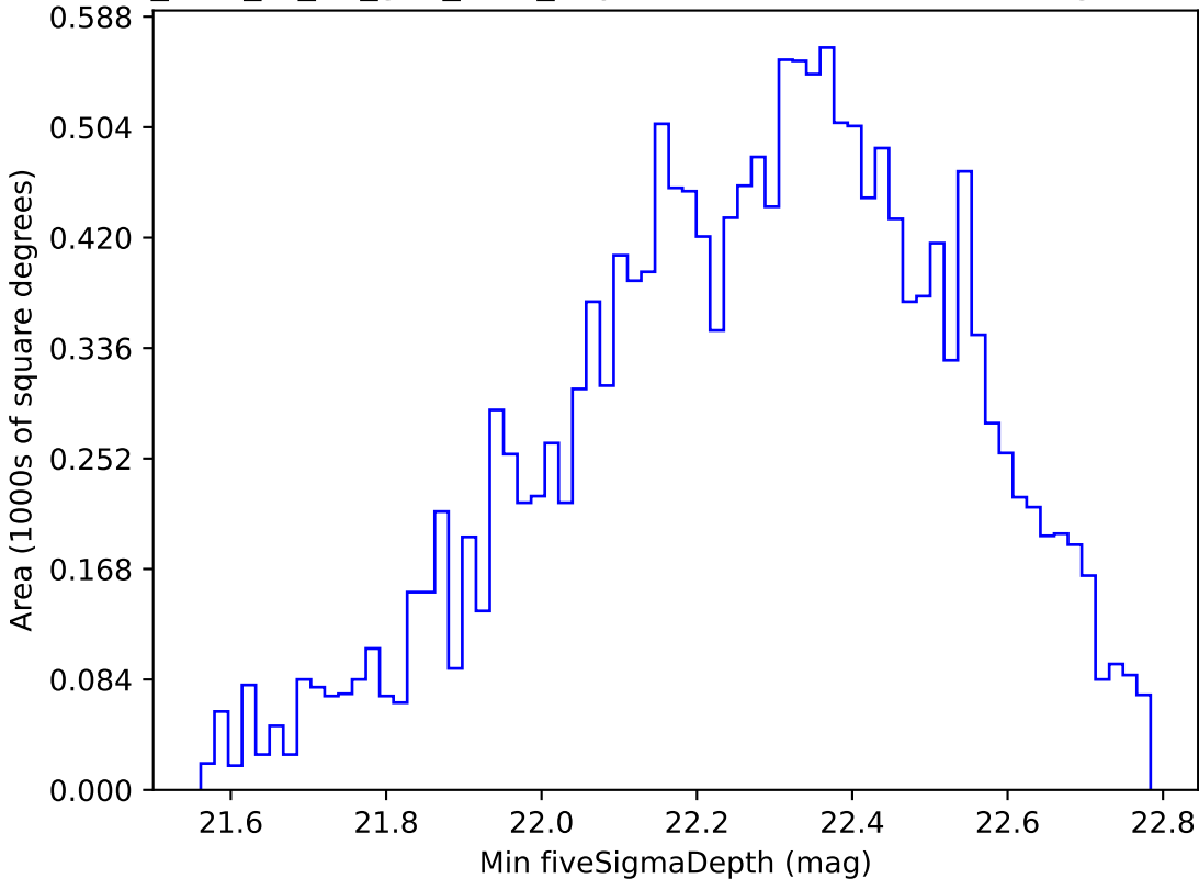
too_elab_r8_d2_griz_v3.4_10yrs WFD u band: Min fiveSigmaDepth
