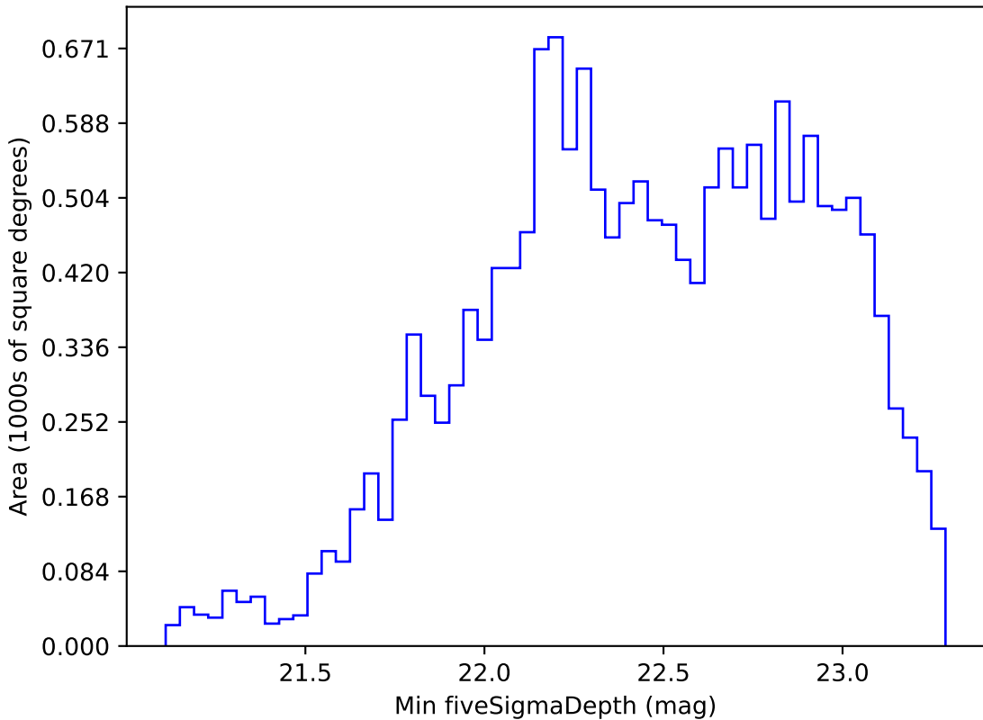
too_elab_r8_d2_griz_v3.4_10yrs WFD r band: Min fiveSigmaDepth
