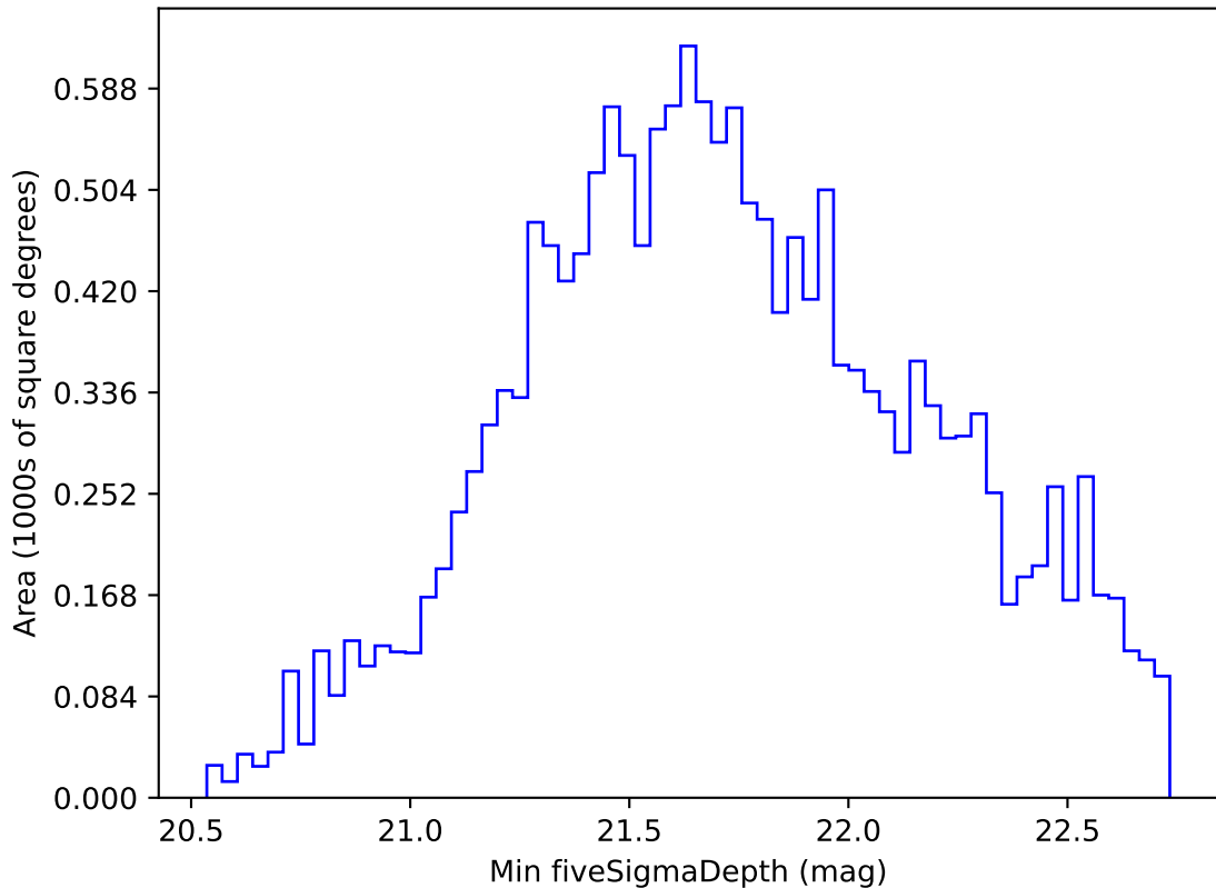
too_elab_r8_d2_griz_v3.4_10yrs WFD i band: Min fiveSigmaDepth
