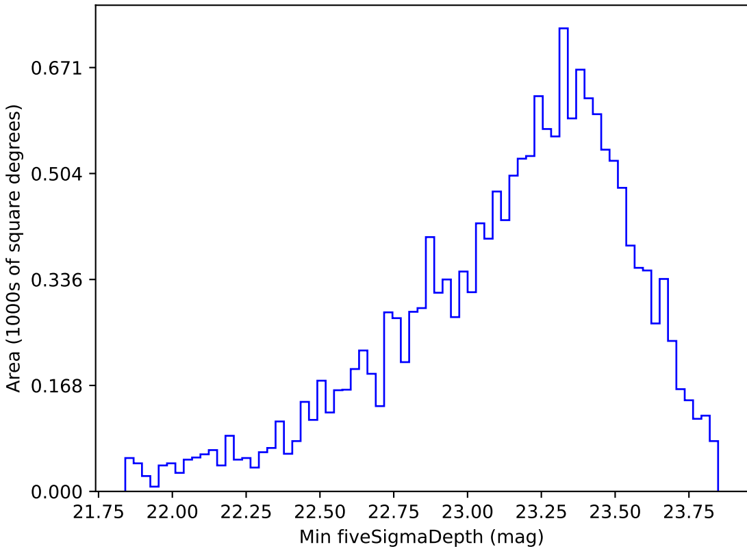
too_elab_r8_d2_griz_v3.4_10yrs WFD g band: Min fiveSigmaDepth
