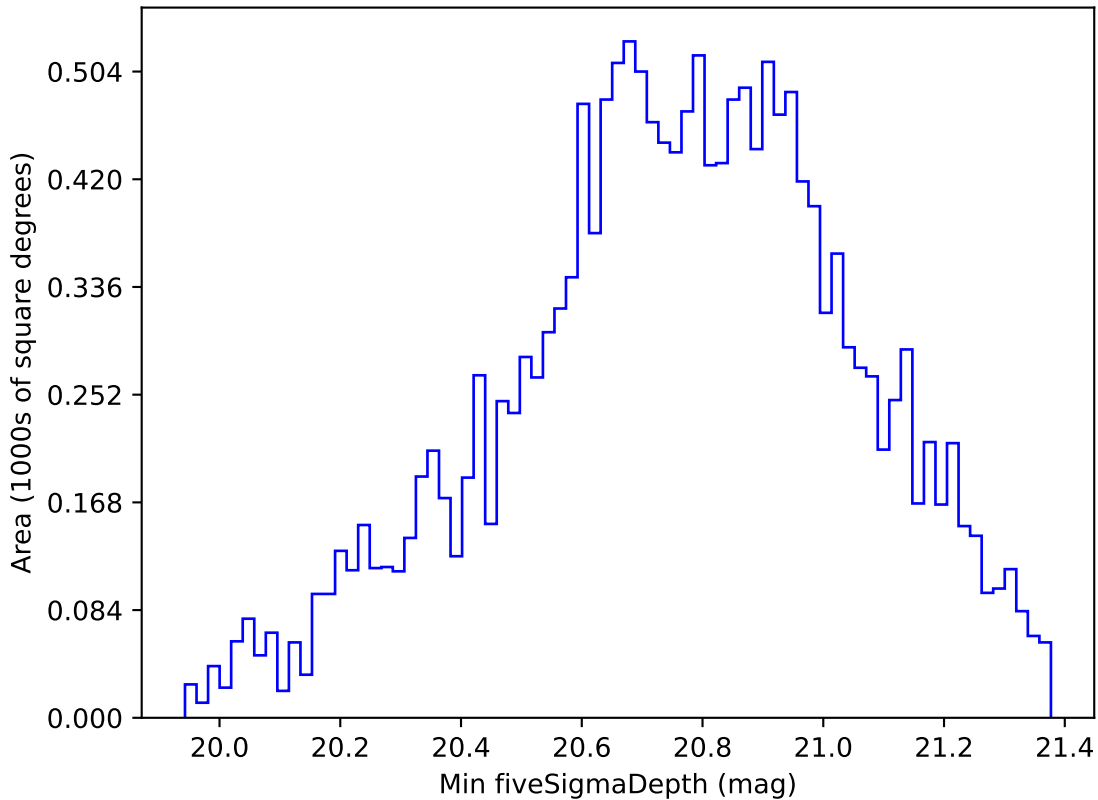
too_elab_r8_d2_griz_v3.4_10yrs WFD all bands: Min fiveSigmaDepth
