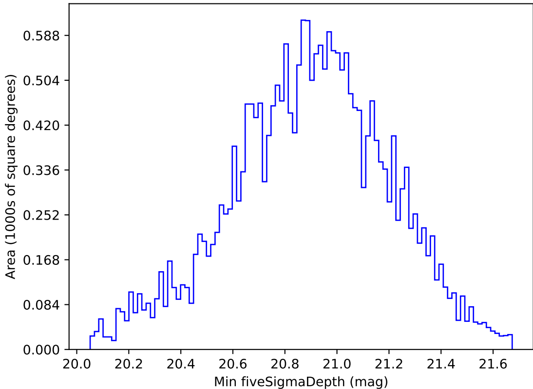
too_elab_r8_d2_griz_v3.4_10yrs All sky y band: Min fiveSigmaDepth
