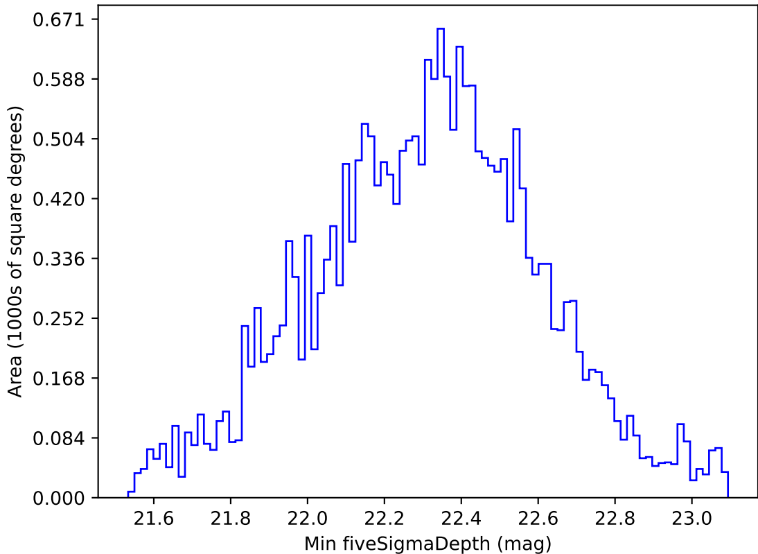
too_elab_r8_d2_griz_v3.4_10yrs All sky u band: Min fiveSigmaDepth
