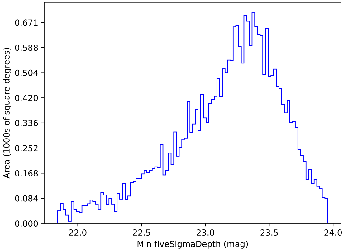
too_elab_r8_d2_griz_v3.4_10yrs All sky g band: Min fiveSigmaDepth
