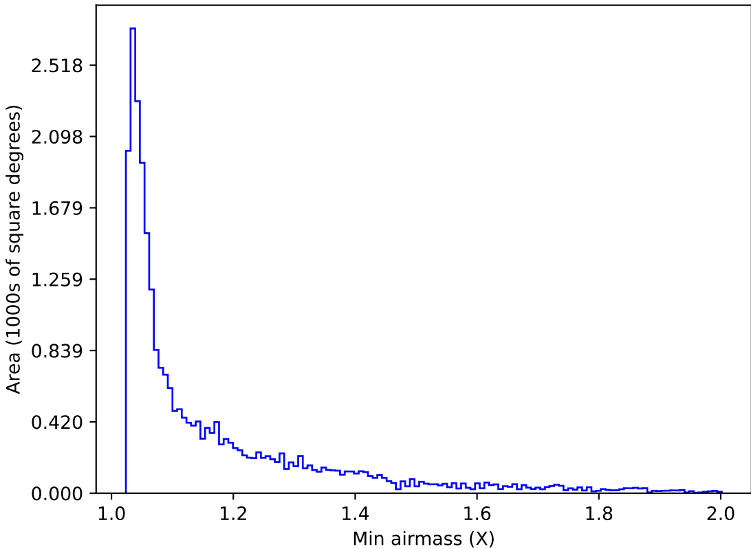
too_elab_r8_d2_griz_v3.4_10yrs Yr 1 z band: Min airmass
