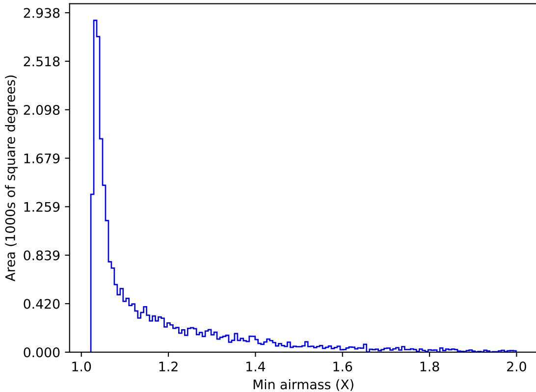
too_elab_r8_d2_griz_v3.4_10yrs Yr 1 r band: Min airmass
