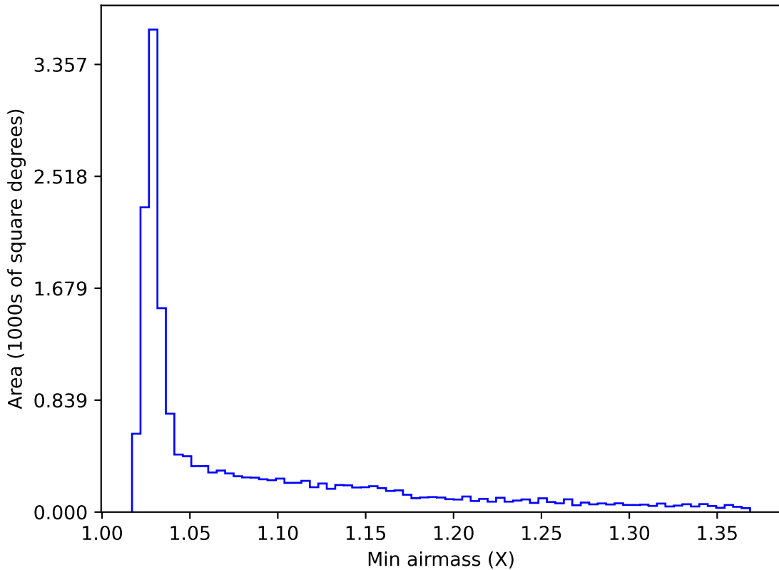
too_elab_r8_d2_griz_v3.4_10yrs WFD z band: Min airmass
