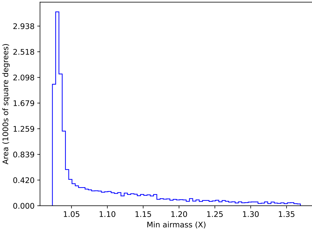
too_elab_r8_d2_griz_v3.4_10yrs WFD y band: Min airmass
