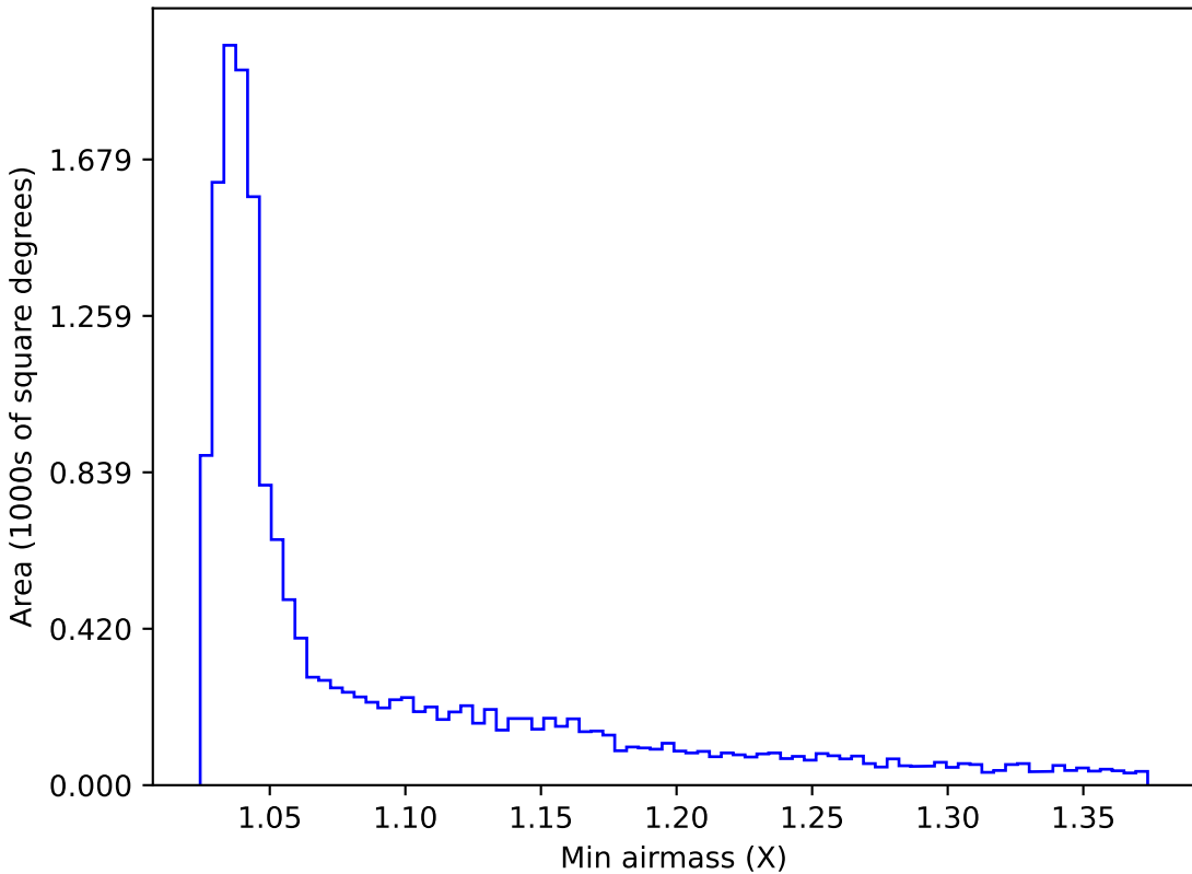
too_elab_r8_d2_griz_v3.4_10yrs WFD u band: Min airmass
