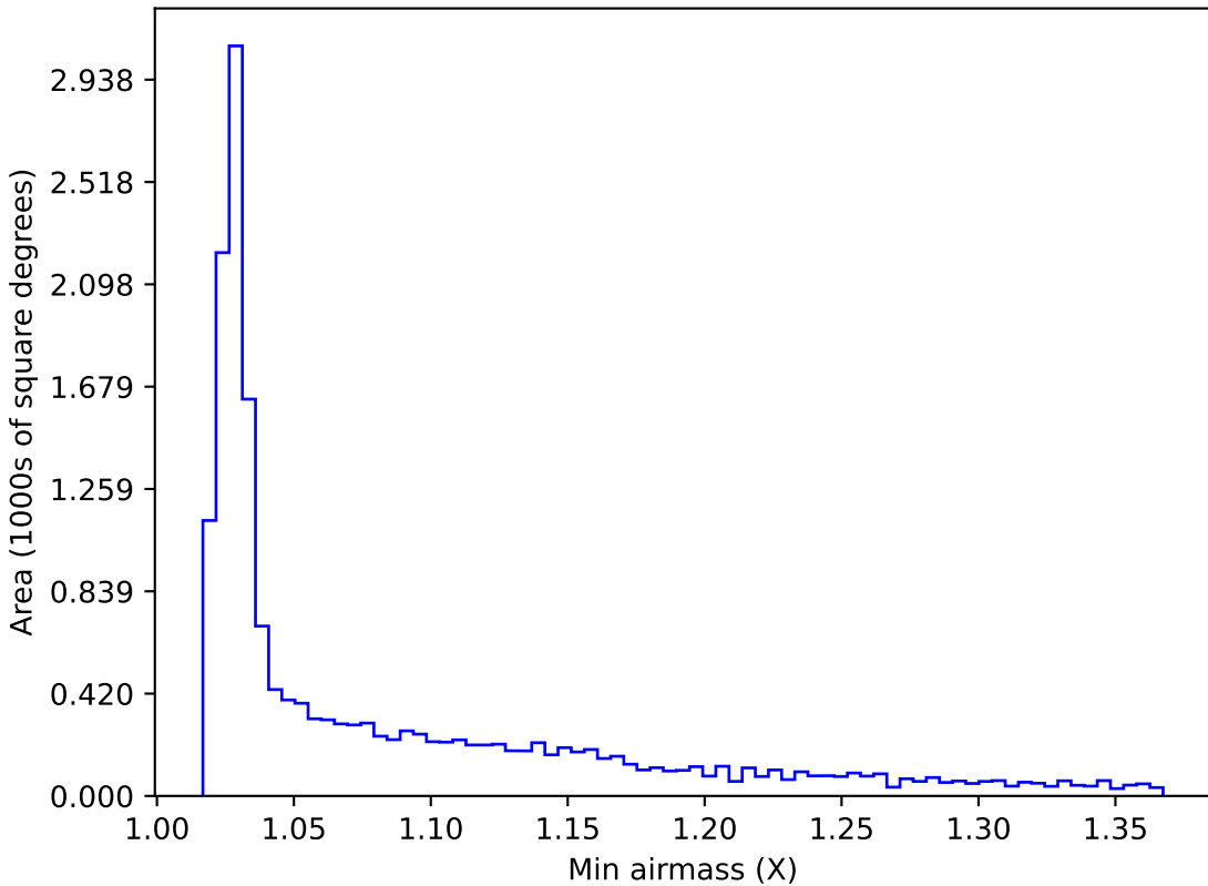
too_elab_r8_d2_griz_v3.4_10yrs WFD r band: Min airmass
