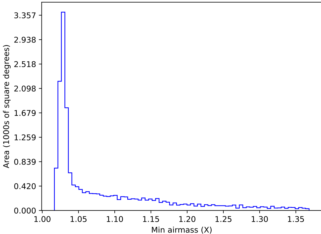
too_elab_r8_d2_griz_v3.4_10yrs WFD i band: Min airmass
