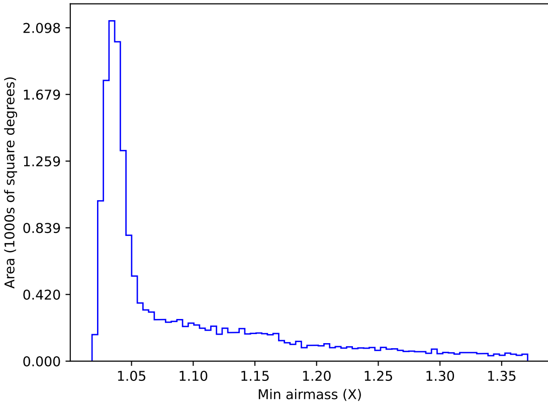
too_elab_r8_d2_griz_v3.4_10yrs WFD g band: Min airmass
