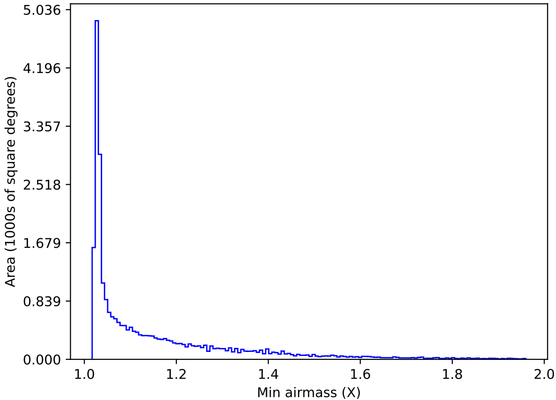
too_elab_r8_d2_griz_v3.4_10yrs All sky i band: Min airmass
