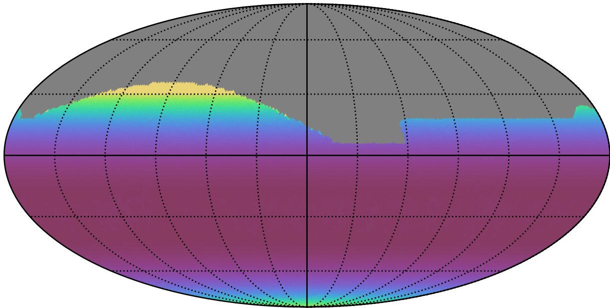
too_elab_r8_d2_griz_v3.4_10yrs All sky all bands: Min airmass
