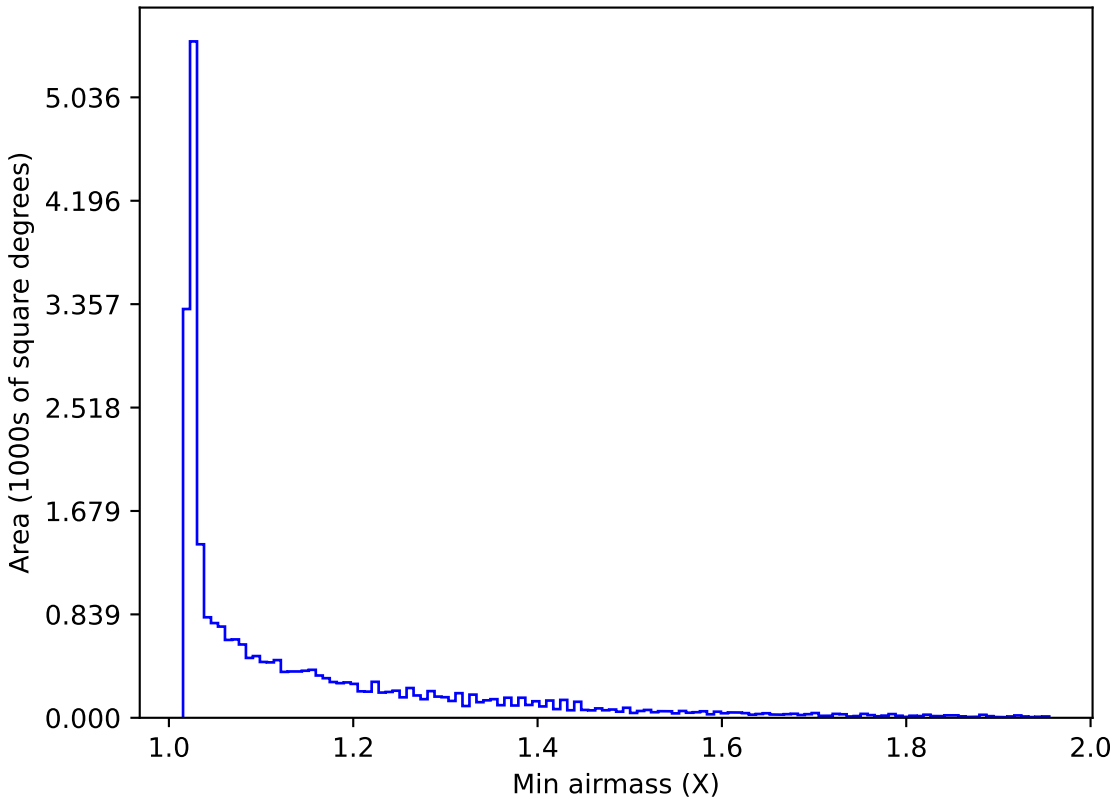
too_elab_r8_d2_griz_v3.4_10yrs All sky all bands: Min airmass
