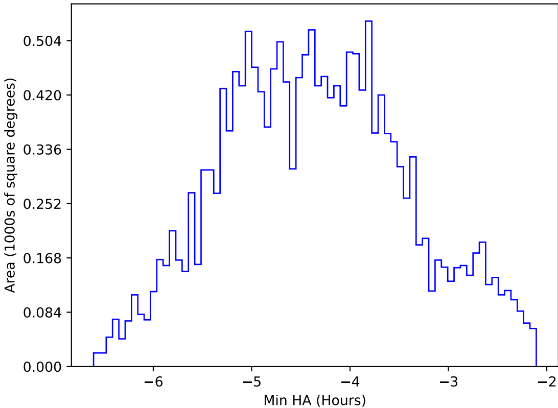
too_elab_r8_d2_griz_v3.4_10yrs WFD z band: Min HA
