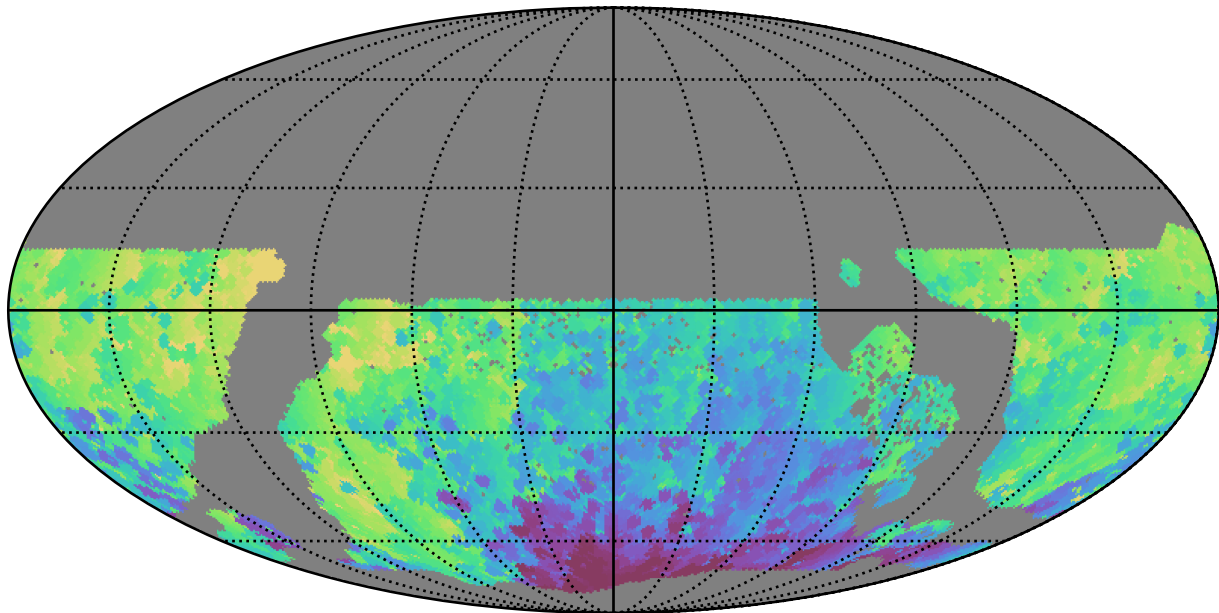
too_elab_r8_d2_griz_v3.4_10yrs WFD y band: Min HA
