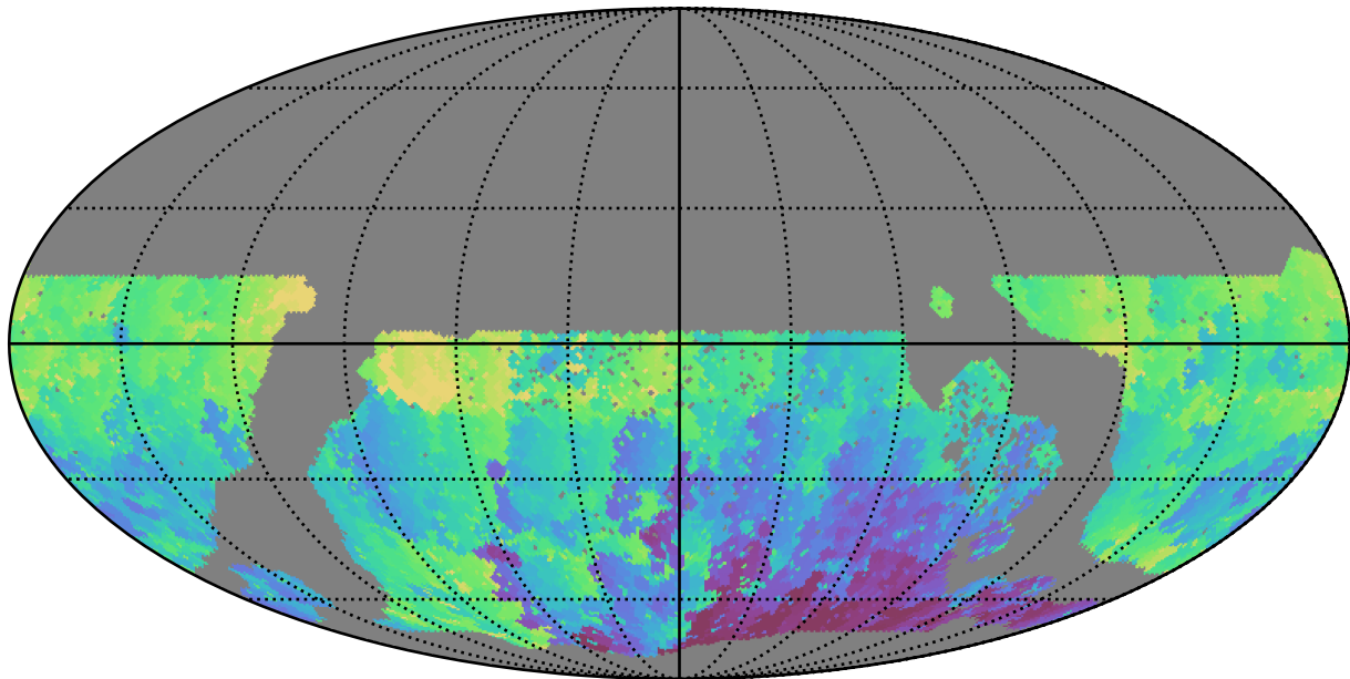
too_elab_r8_d2_griz_v3.4_10yrs WFD u band: Min HA
