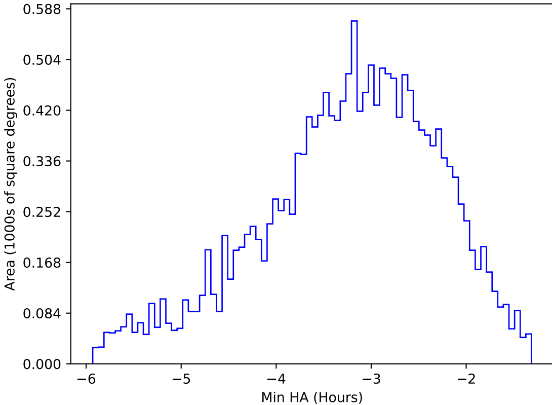
too_elab_r8_d2_griz_v3.4_10yrs WFD u band: Min HA
