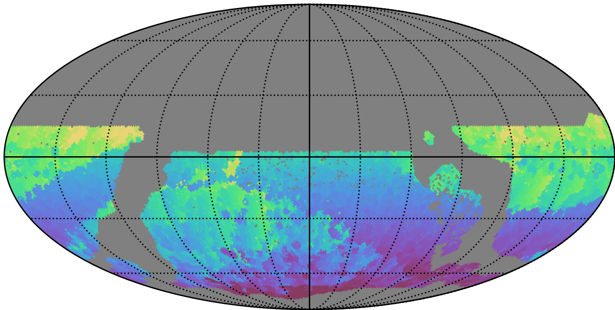
too_elab_r8_d2_griz_v3.4_10yrs WFD r band: Min HA
