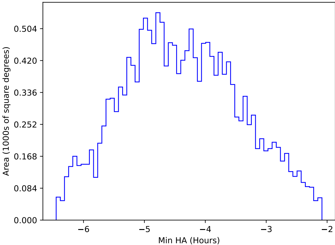
too_elab_r8_d2_griz_v3.4_10yrs WFD i band: Min HA
