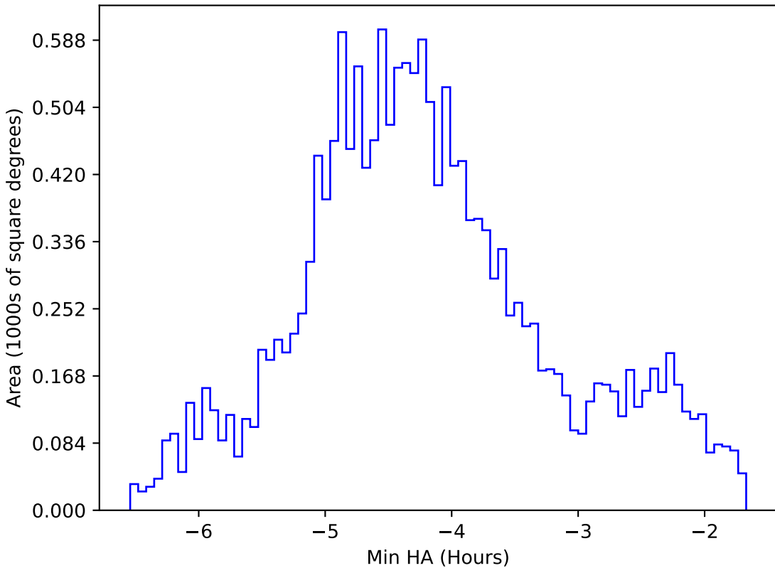
too_elab_r8_d2_griz_v3.4_10yrs WFD g band: Min HA
