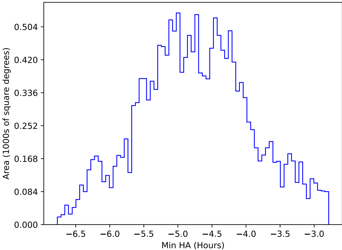
too_elab_r8_d2_griz_v3.4_10yrs WFD all bands: Min HA
