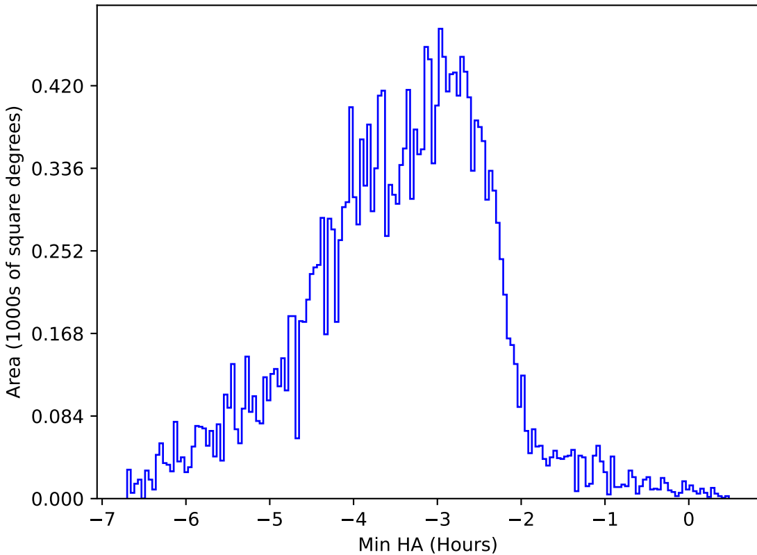
too_elab_r8_d2_griz_v3.4_10yrs All sky y band: Min HA
