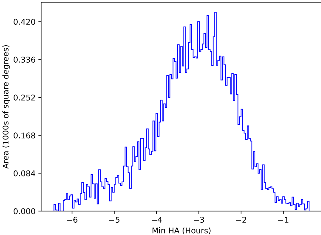
too_elab_r8_d2_griz_v3.4_10yrs All sky u band: Min HA
