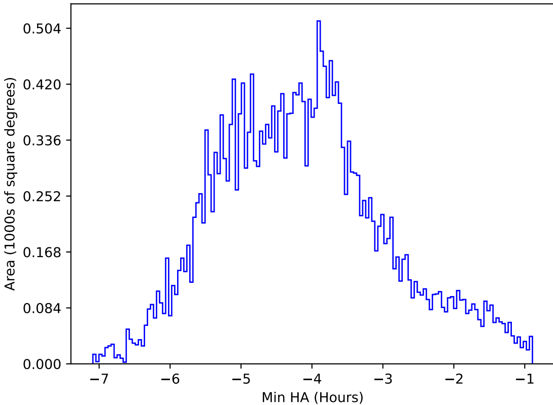
too_elab_r8_d2_griz_v3.4_10yrs All sky r band: Min HA
