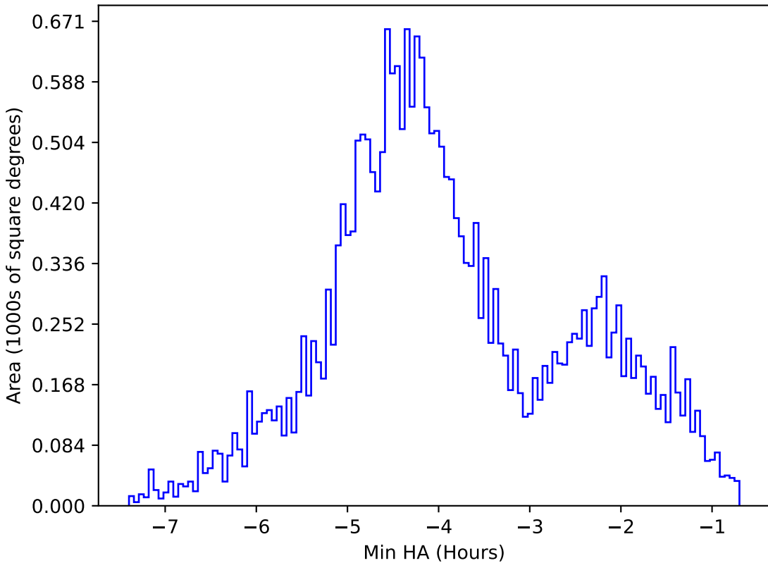
too_elab_r8_d2_griz_v3.4_10yrs All sky g band: Min HA
