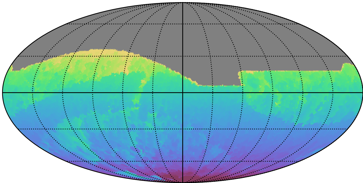
too_elab_r8_d2_griz_v3.4_10yrs All sky all bands: Min HA
