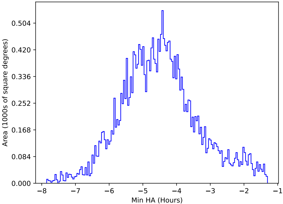
too_elab_r8_d2_griz_v3.4_10yrs All sky all bands: Min HA
