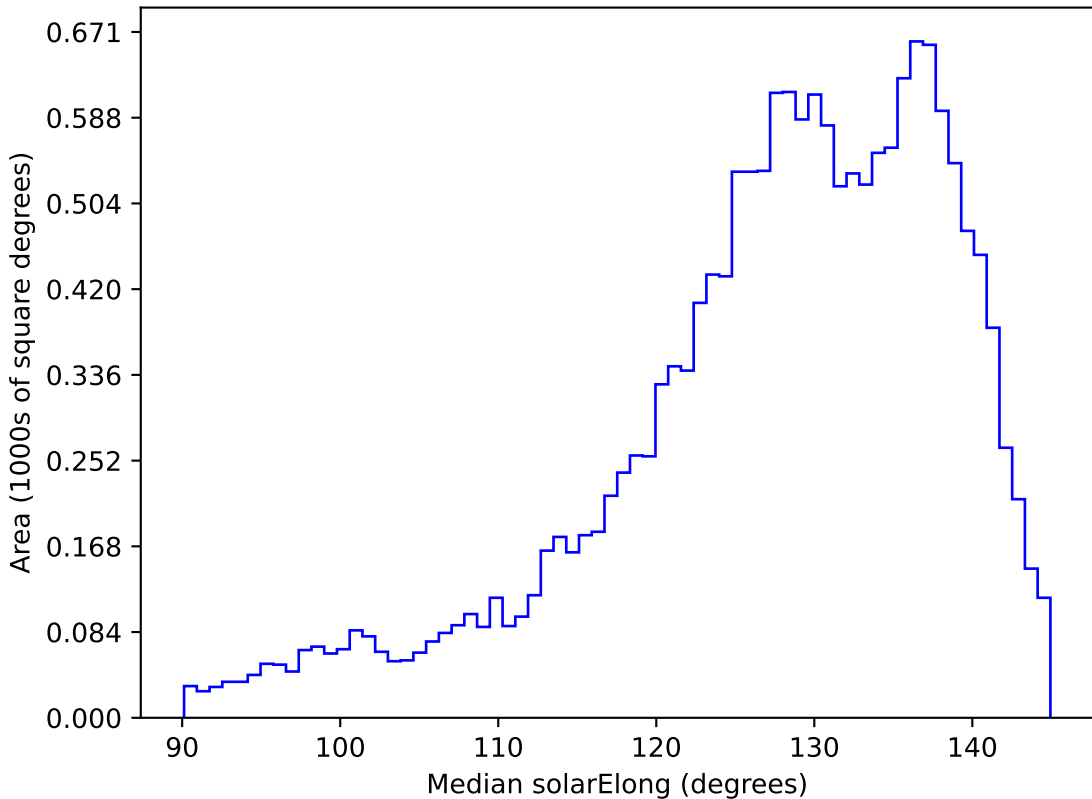
too_elab_r8_d2_griz_v3.4_10yrs WFD z band: Median solarElong
